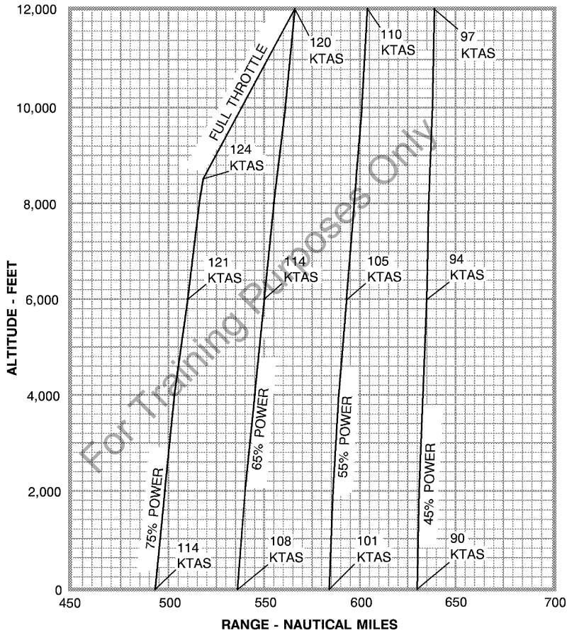
Figure 5-9. Range Profile
